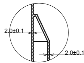
DETAIL E SCALE 1:2
