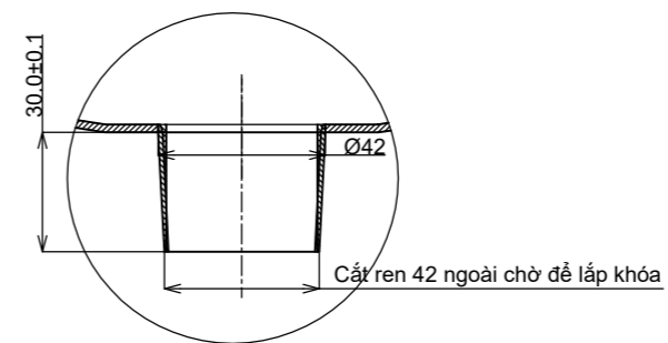
DETAIL H SCALE 1:2
